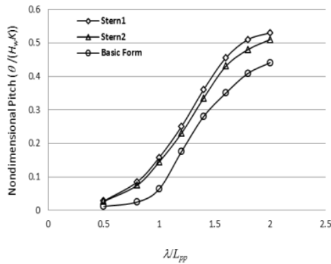
Figure 12 Non-dimensional pitch motions of each stern part improvement
