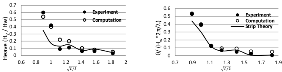
Figure 2 Transfer function of heave motions and pitch motions of the tanker
