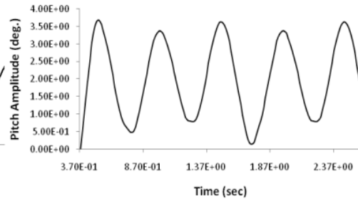
Figure 9 Time history of pitch amplitude of Stern1 ( Fr=0.384 , \lambda/L_{pp}=1.2 , H_w/L_{pp}=0.06 )
