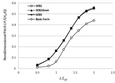
Figure 13 Non-dimensional pitch motions of each addition structure attachment
